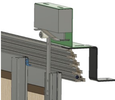
Gate Closure Switch, Bracket, & Gate Arm
